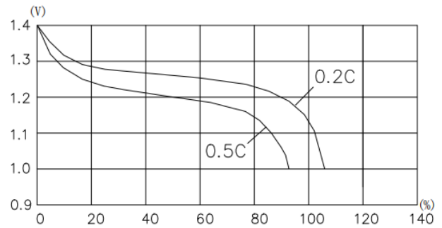
Discharge Curve at Different Rate (20°C)
